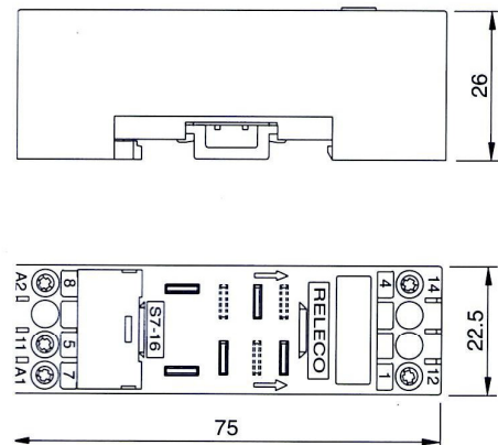
S7-16 for relays C7-A10 (16 A)
